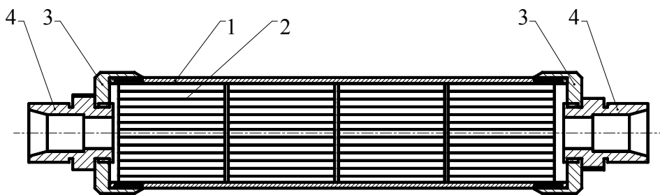
Figure 3. Reinforced Thermal Register
