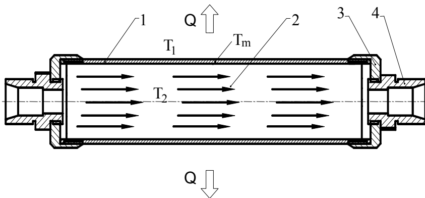
Figure 2. Simple thermal register
