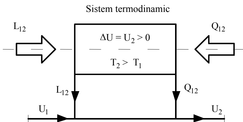
Figure 1. The energy fluxes in a thermodynamic system
